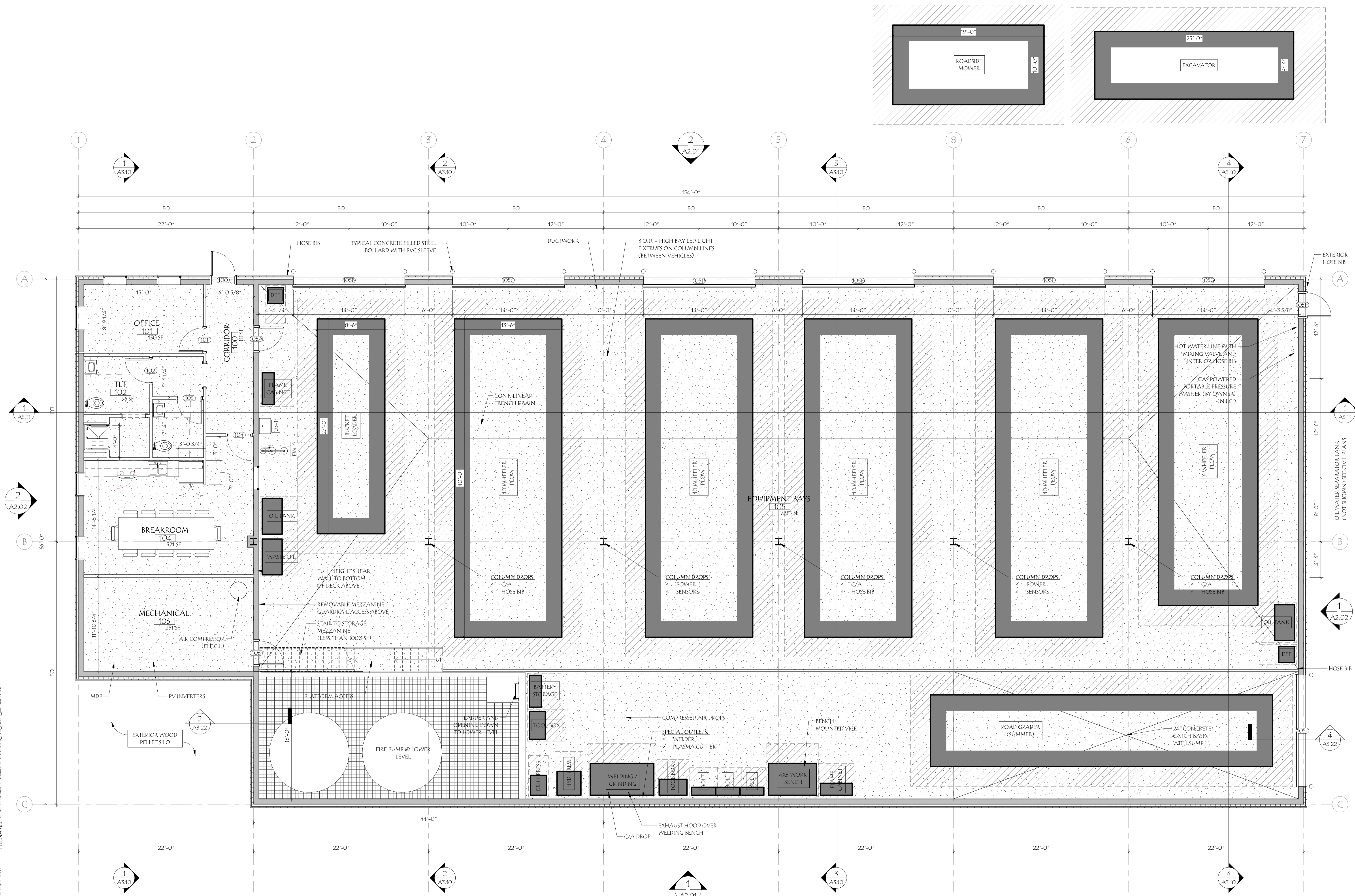
1 PROPOSED OVERALL LEVEL 1 PLAN SD-01 3/16" = 1'-0"
